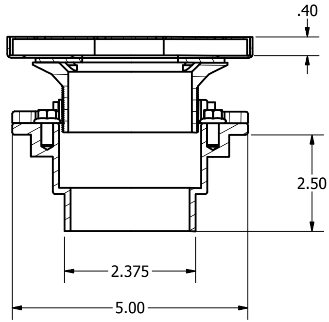
SECTION E-E SCALE 1 / 2
