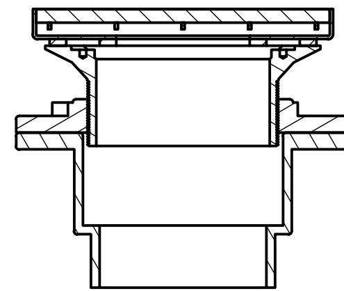
SECTION D-D SCALE 1 / 2
